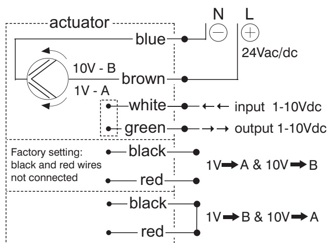
Wiring diagram M07 0–10 V
