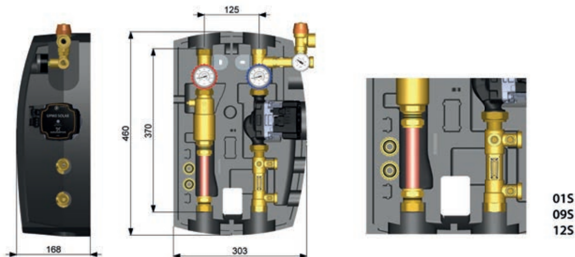
Dimensions of groups with copper pipe (01S-09S-12S) - Detail of groups with copper pipe
