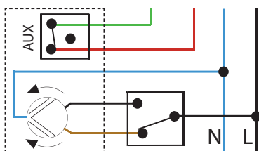
Wiring diagram M01, 3 points with aux. microswitch
